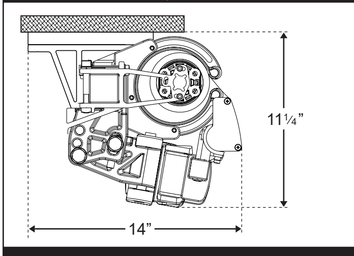
TOTAL ECLIPSE - Soffit Mount (no hood option available)
