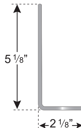
5" No Cassette Bracket - Side View
