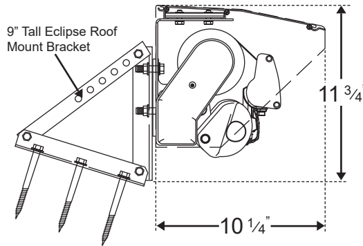
ECLIPSE PREMIER - Roof Mount
