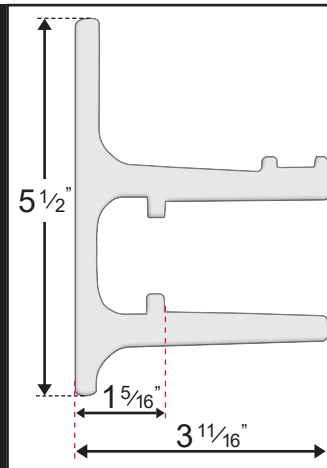
Wall Bracket - Side View
