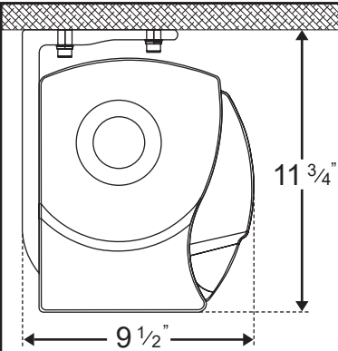
ECLIPSE PREMIER with SC - Soffit Mount
