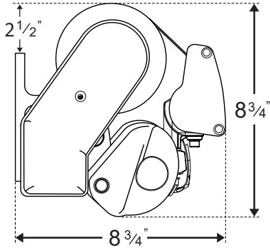
ECLIPSE PREMIER - Wall Mount (no hood)
