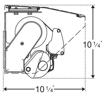
ECLIPSE PREMIER - Wall Mount (with hood)
