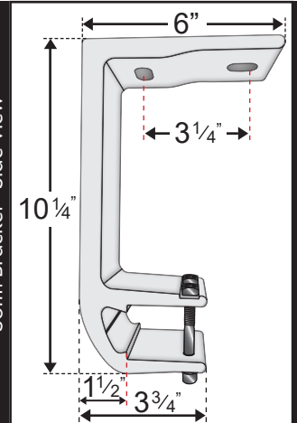
Soffit Bracket - Side View
