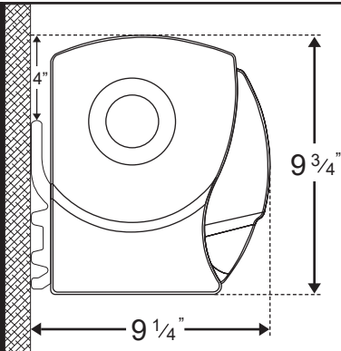
ECLIPSE PREMIER with SC - Wall Mount
