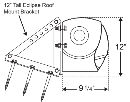
ECLIPSE PREMIER with SC - Soffit Mount
